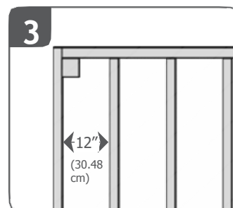
Diagonal (45 degree) Installation Substructure 12" (30.48 cm) on center maximum joists. Different angles will require – 60 degrees 14" (35.56 cm) on center spacing, 30 degrees 6" (15.24 cm) on center. (Building codes may vary by location.)
